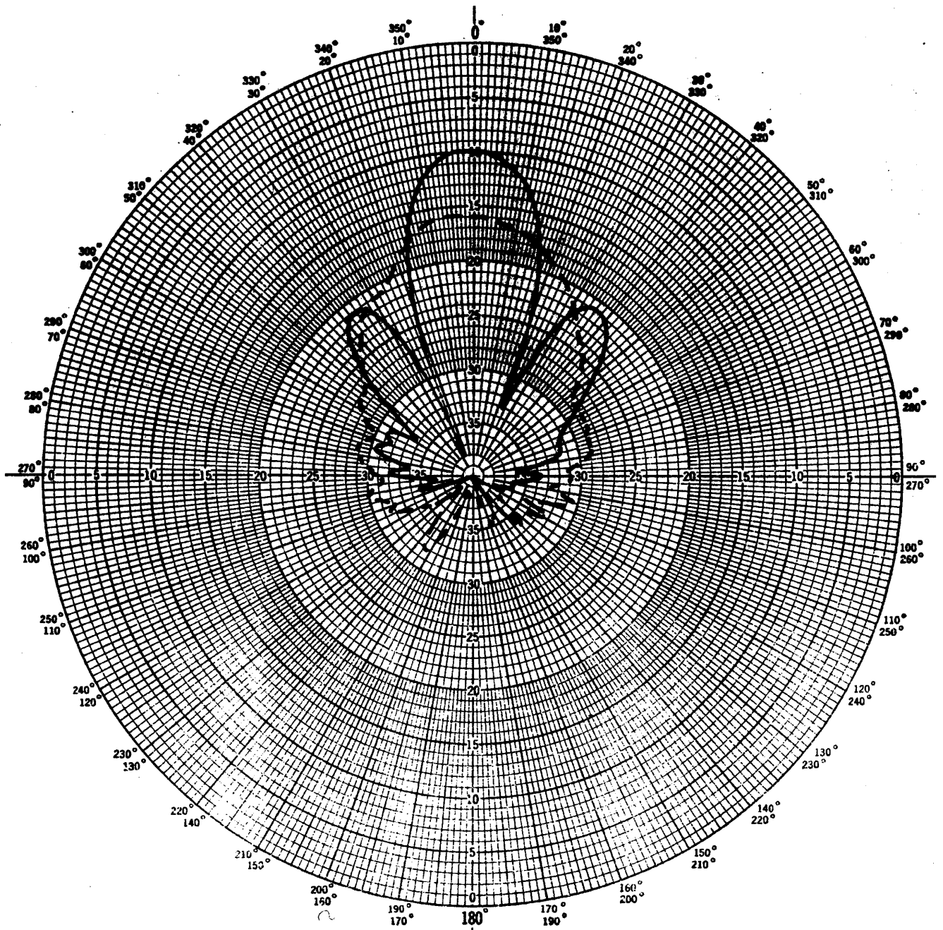
E PLANE RADIATION PATTERN 9.0 GHz
