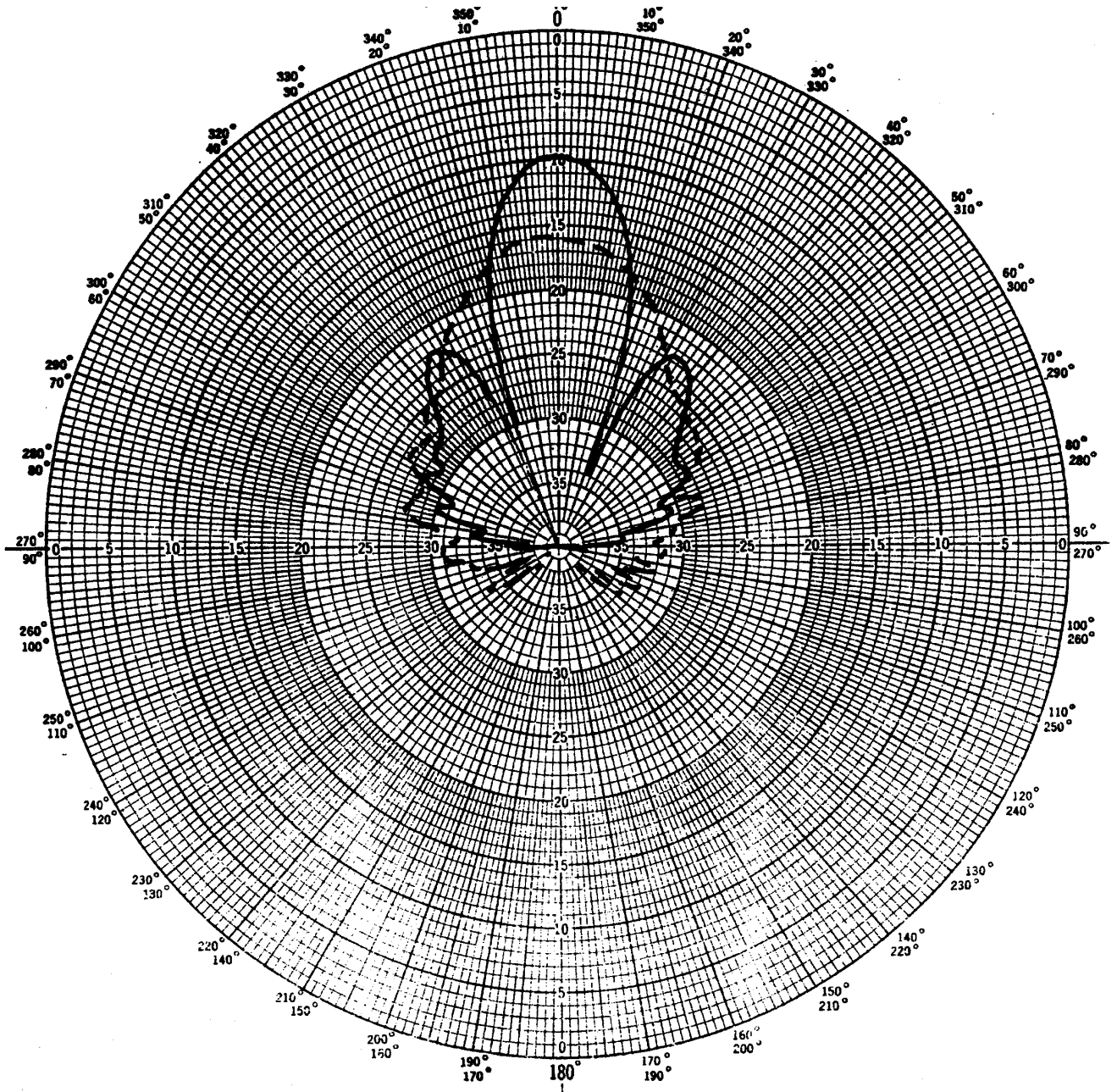
E PLANE RADIATION PATTERN 10.0 GHz
