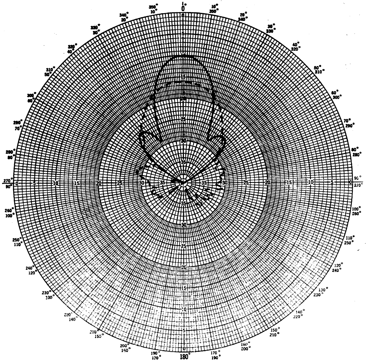
E PLANE RADIATION PATTERN 8.0 GHz
