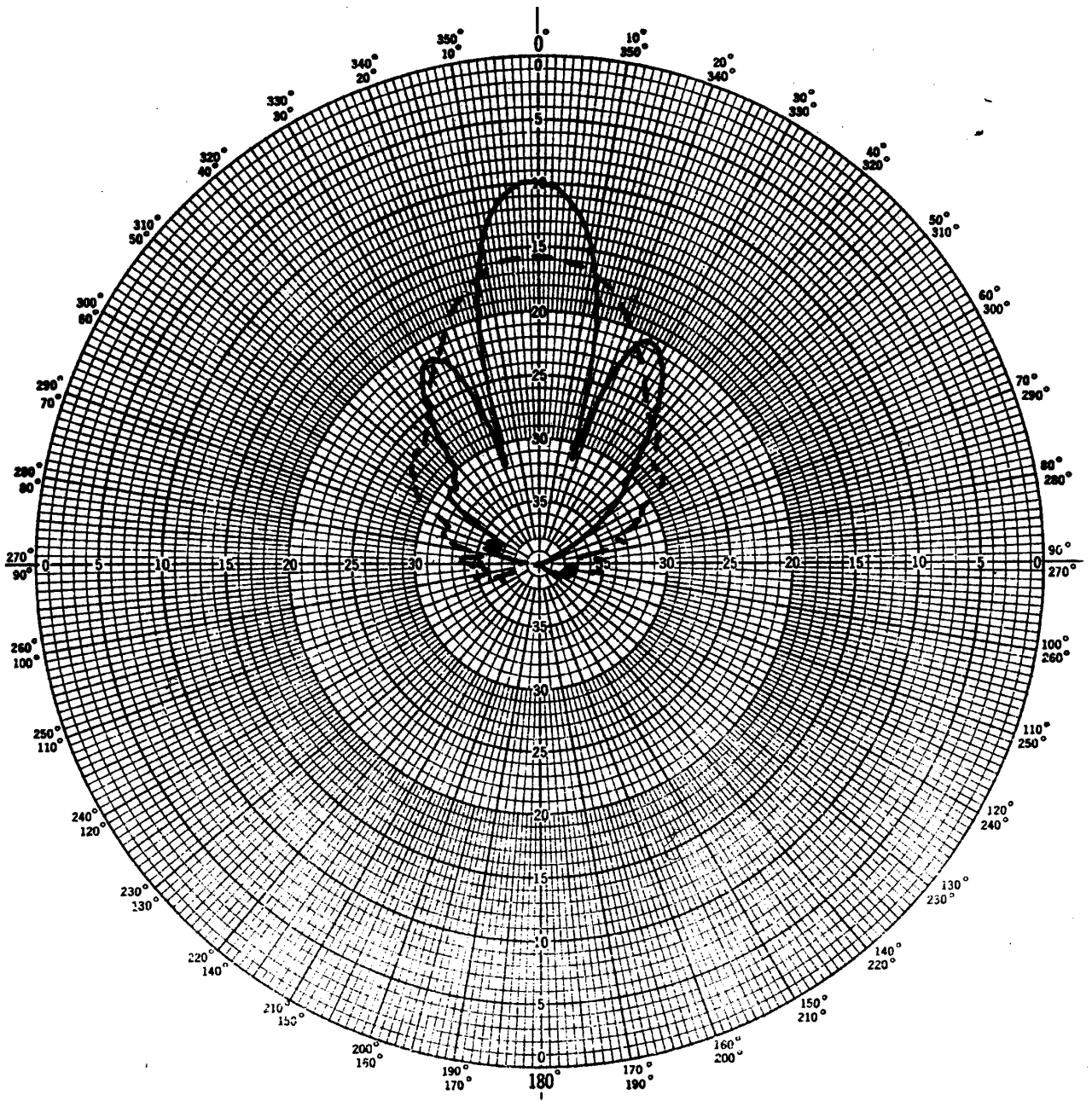
E PLANE RADIATION PATTERN 12.0 GHz
