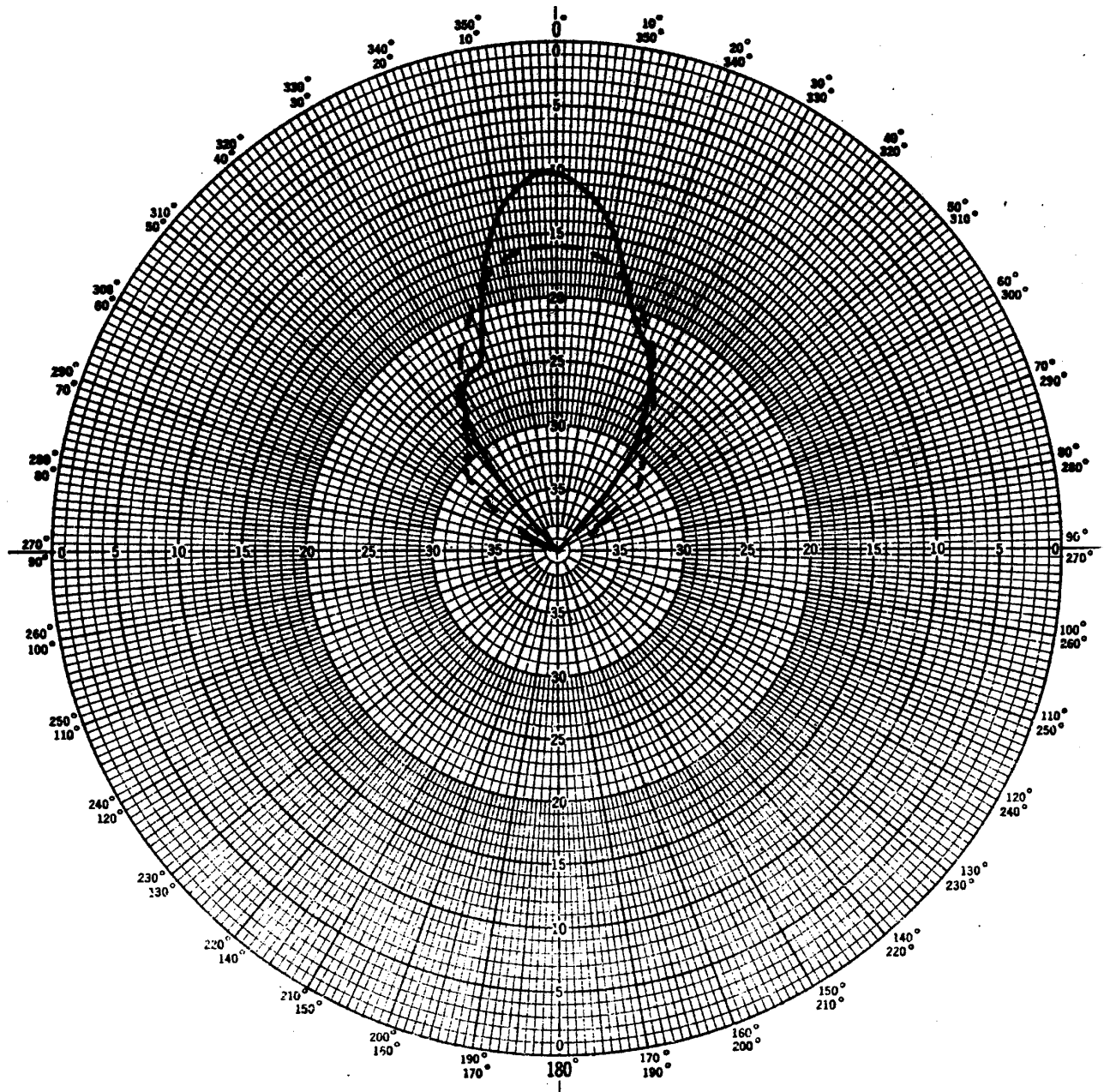
H PLANE RADIATION PATTERN 12.0 GHz
