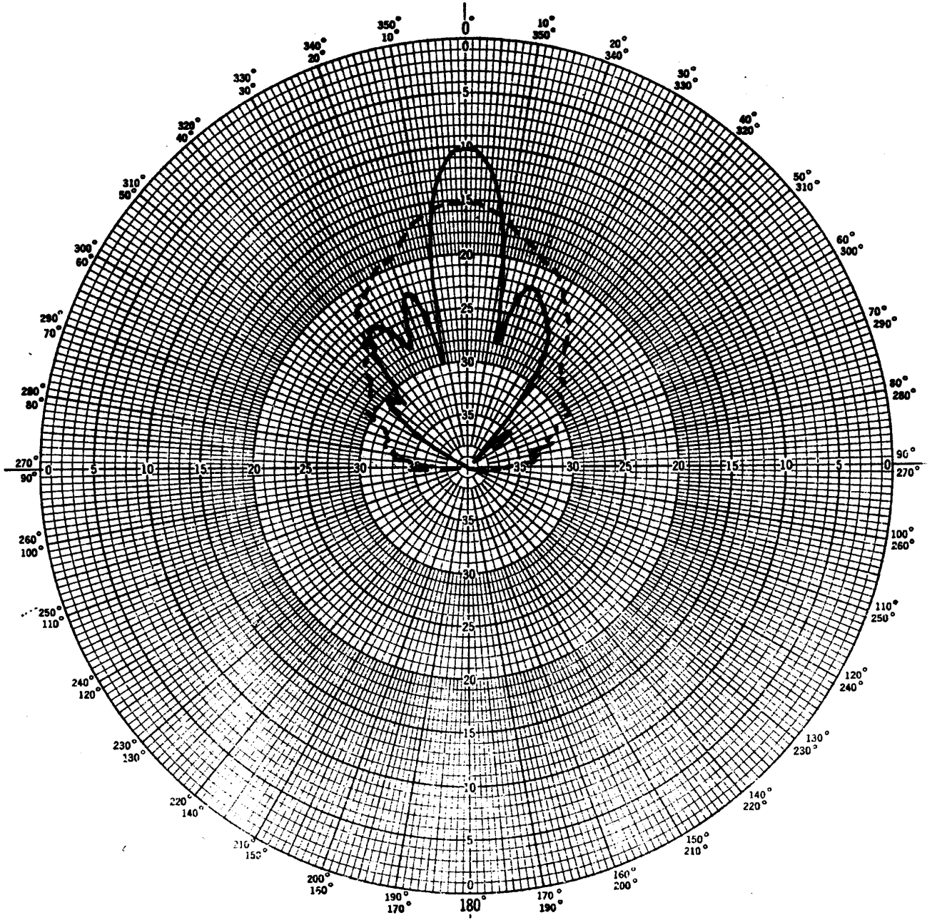
E PLANE RADIATION PATTERN 18.0 GHz
