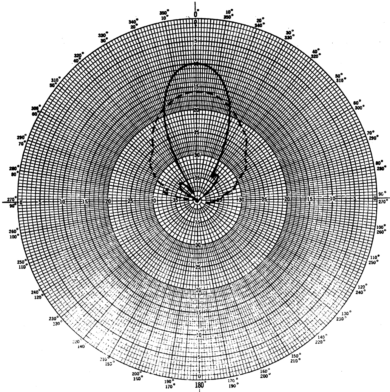
H PLANE RADIATION PATTERN
