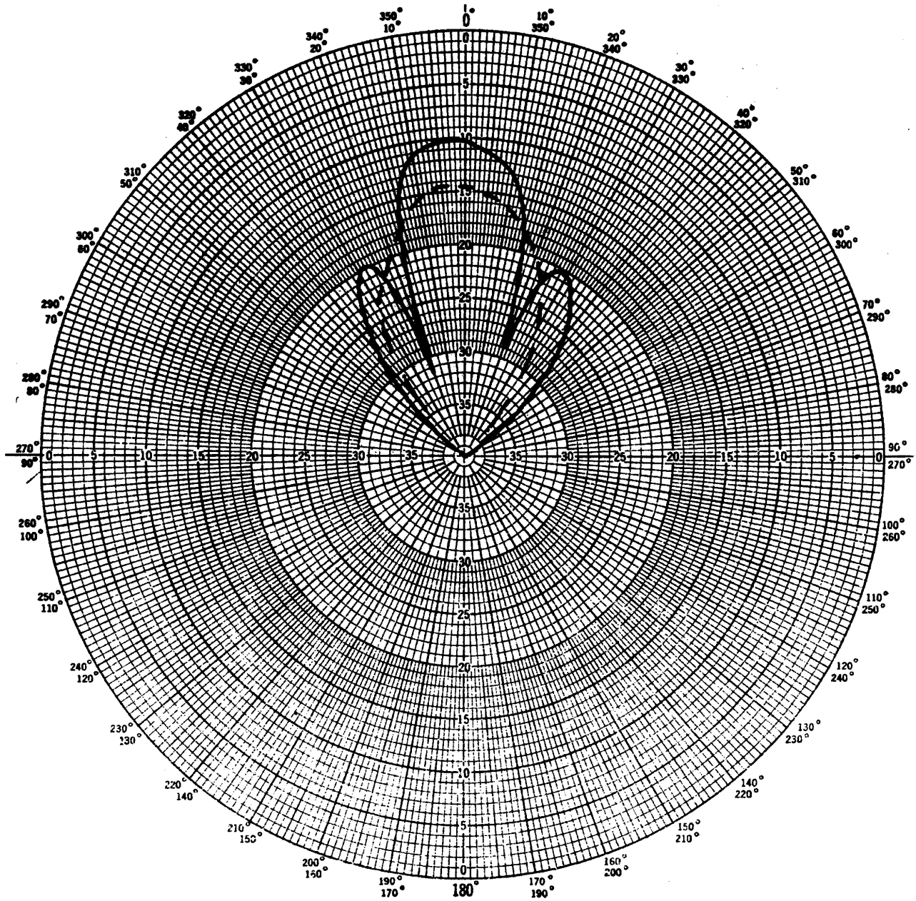
H PLANE RADIATION PATTERN 18.0 GHz
