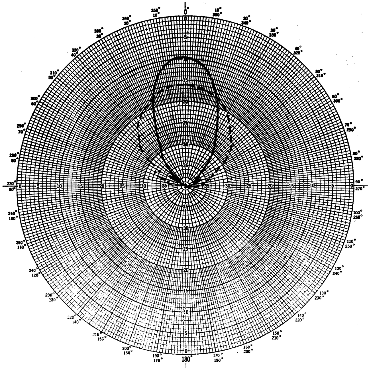
H PLANE RADIATION PATTERN 9.0 GHz
